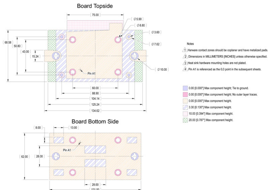
Figure 8. Motherboard Component-Height Restrictions for Custom 2U-4P Systems
